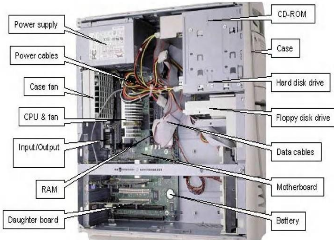
Inside view of System Unit
